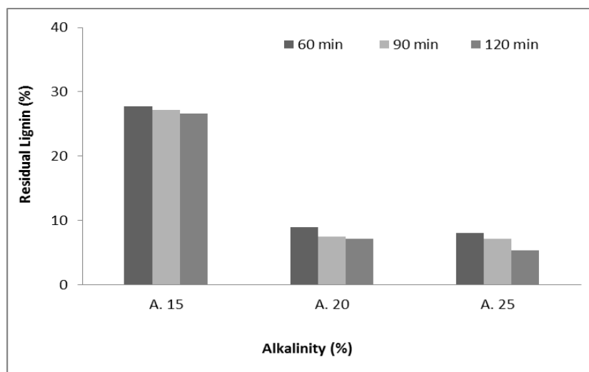
Figure 1. The effects of alkalinity and cooking time on the residual lignin in Kraft pulp
